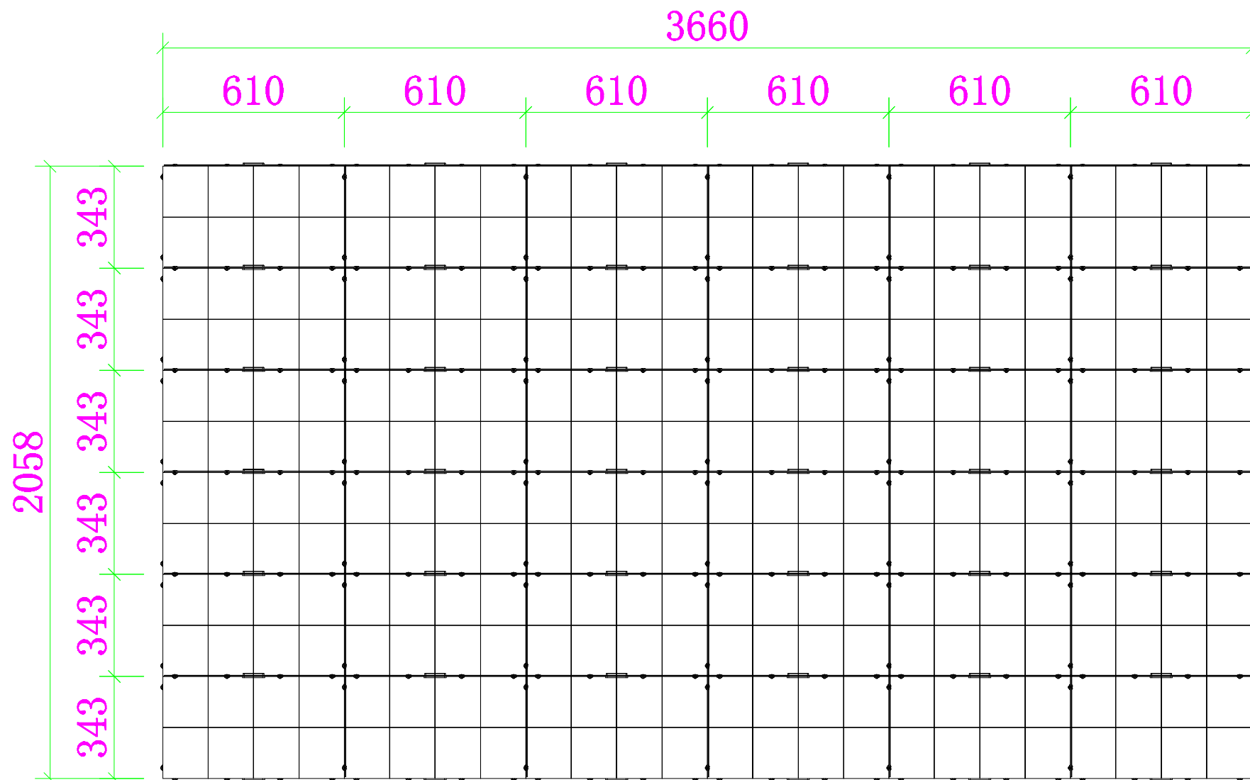
Front view
