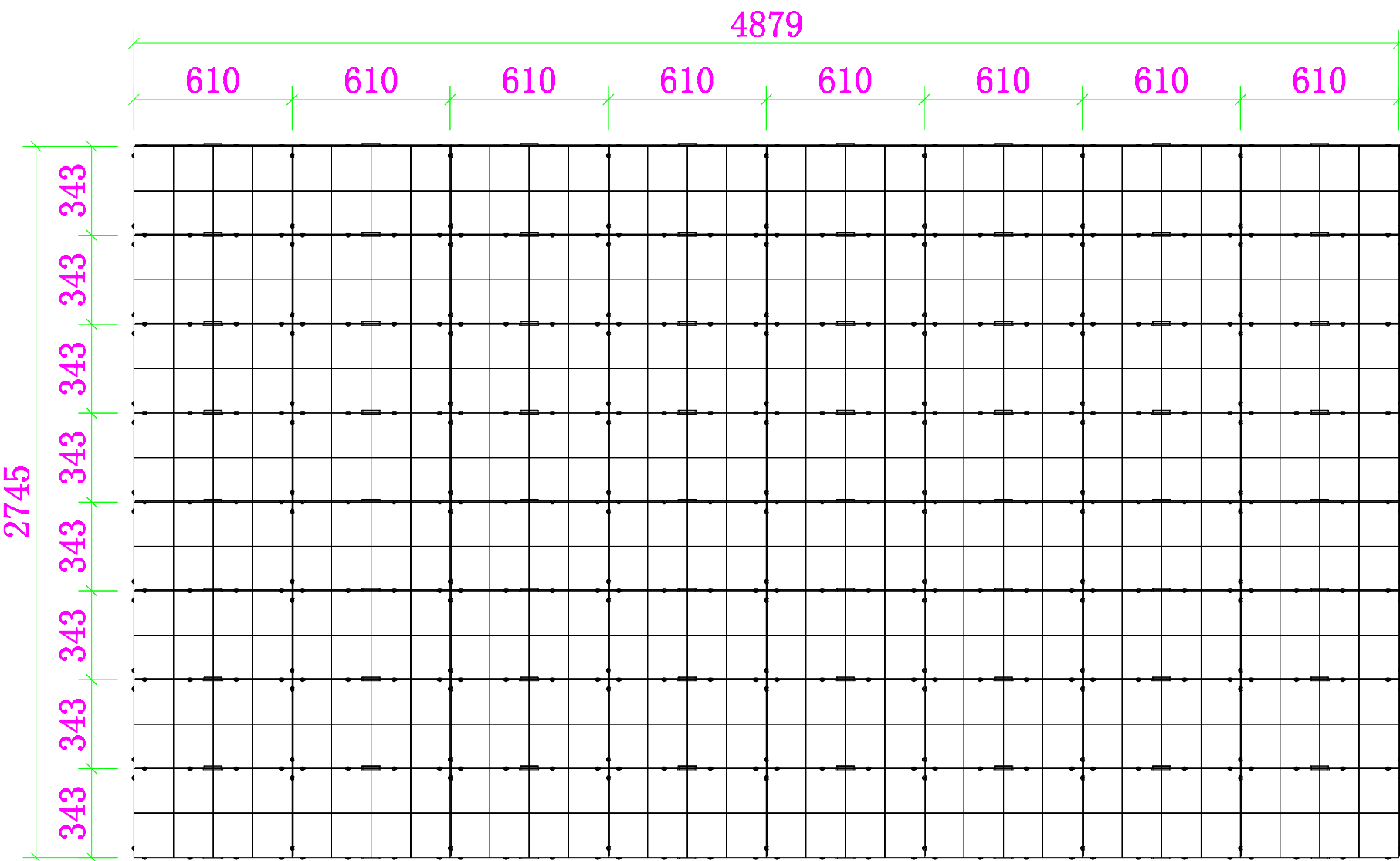
Front view
